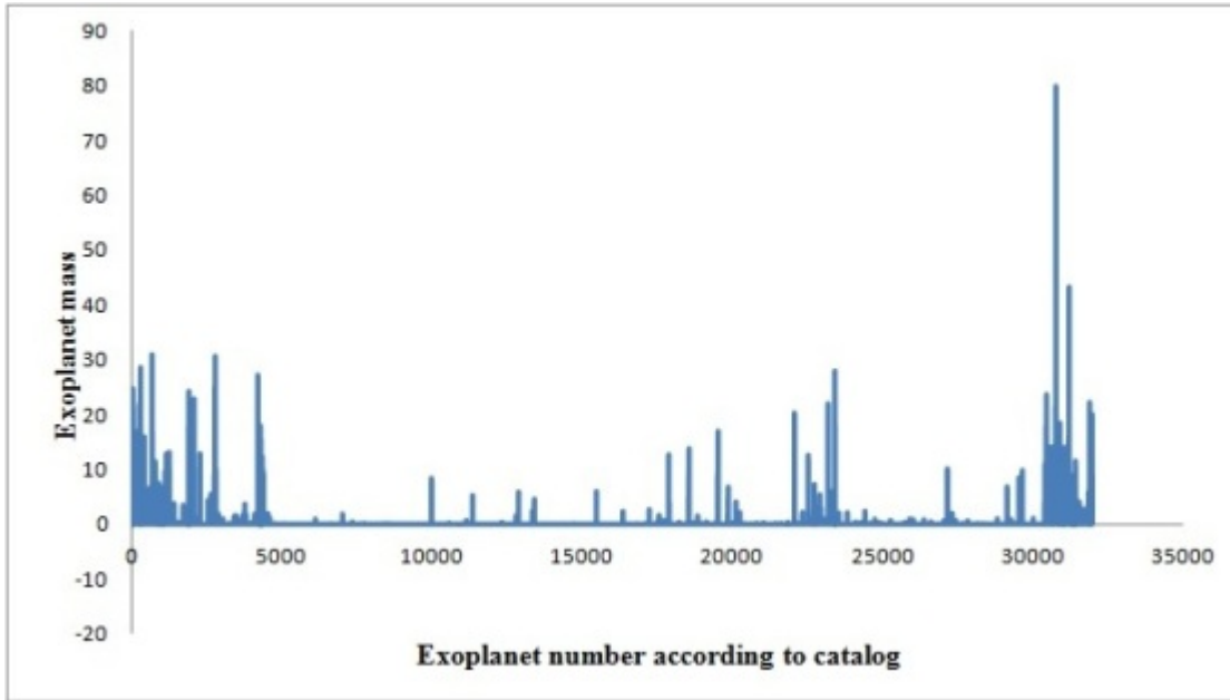
Fig. 1. Distributions of exoplanets by their masses according to the NASA Exoplanet Archive catalog, expressed in Jupiter masses.
