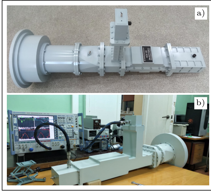
Fig. 1. Dual-band (13 and 25 cm) decimeter-wave antennas: (a) development of SKARD-Electronics, Kursk; (b) development of the Special Design Bureau of the Institute of Radioengineering and Electronics of the Russian Academy of Science.
