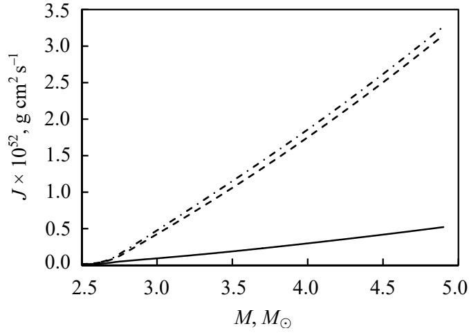
Fig. 2. Angular momentum brought by accreted matter in cases where A_0 = 30 R_\odot (dot-dashed line) and A_0 = 15 R_\odot (dashed line), and angular momentum of the accretor (solid line) as functions of its mass.
