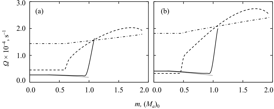
Fig. 1. Angular velocity in the interior of the accretor before the mass exchange (dotted line), when the surface receives Kepler rotation (solid line), at the end of the mass exchange (dashed line), and after relaxation towards thermal equilibrium (dot-dashed line) in the cases where the initial mass of the accretor is (M_a)_0 = 5 M_\odot (a) and (M_a)_0 = 2.5 M_\odot (b).
