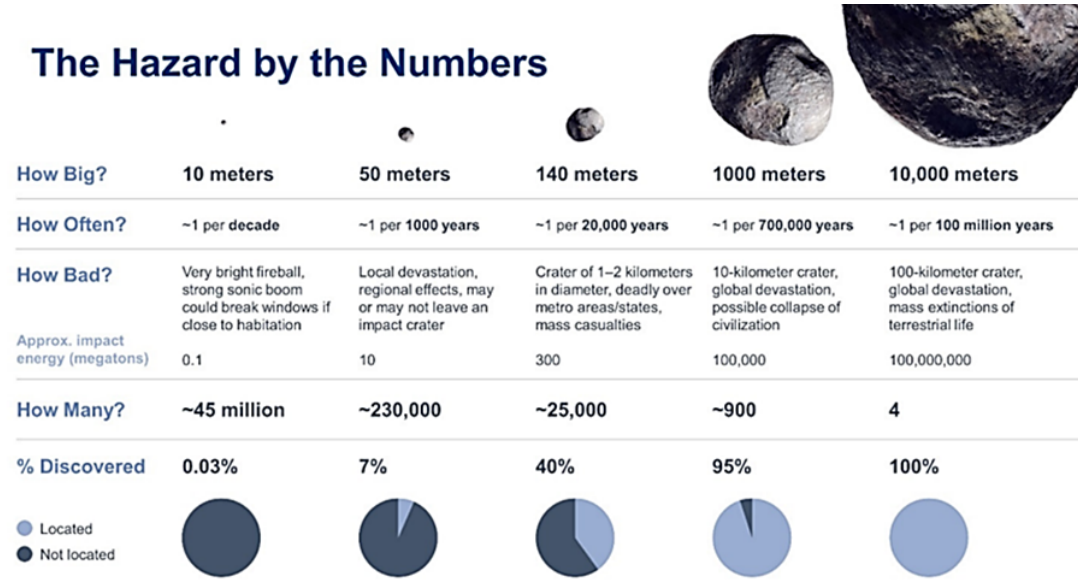
Fig. 1. NEO size, frequency of Earth-impact, and hazard
