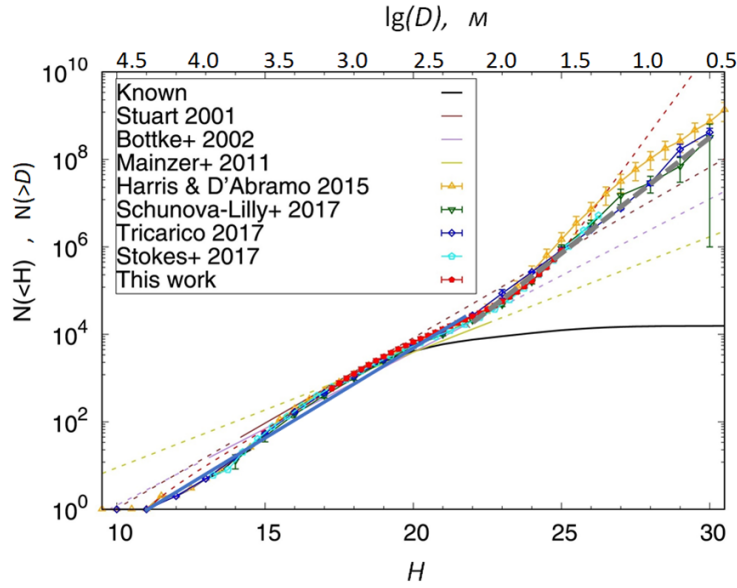
Fig. 3. The observed cumulative distribution of NEOs by H (also by diameter D ) according to the model of Granvik et al. (2018) (marked as 'This work'), and models presented by other authors.
