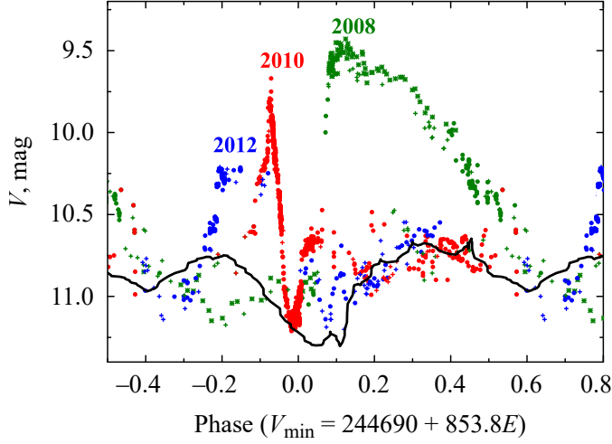
Fig. 1. Phase curves of outburst 2008, 2010, 2012. A solid black curve depicts the phase curve of a star in a quite state.
