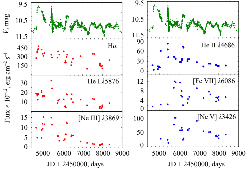
Fig. 2. Light curve in V -band and variation of line fluxes.
