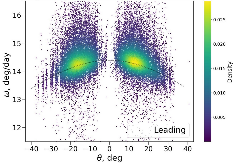
Fig. 1. Scatter plot of the rotation rate of sunspots of the leading magnetic polarity. The dotted line shows the rotation rate according to (Newton & Nunn 1951).
