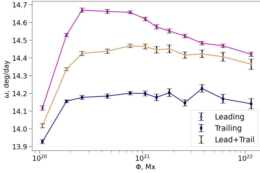
Fig. 3. Rotation rate of sunspots of different magnetic polarity depending on their magnetic flux with latitude in the range \theta : \pm 15^\circ .
