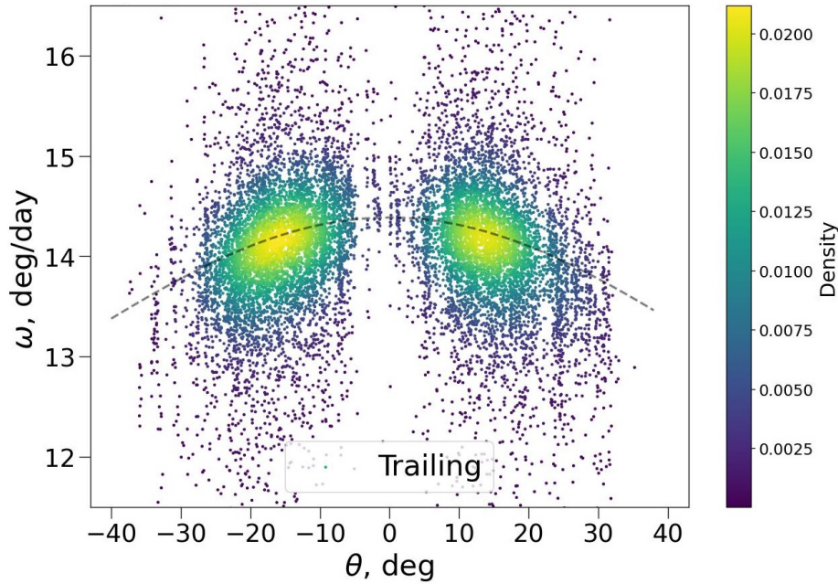
Fig. 2. Same as in Fig. 1 but for sunspots of trailing polarity.
