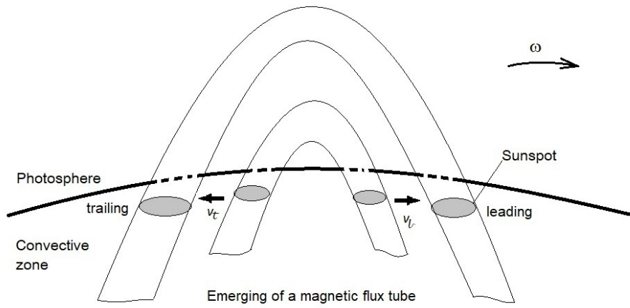
Fig. 4. Simplified diagram of the possible formation of additional speed of longitudinal displacement of sunspots during the emergence of a magnetic flux tube.
