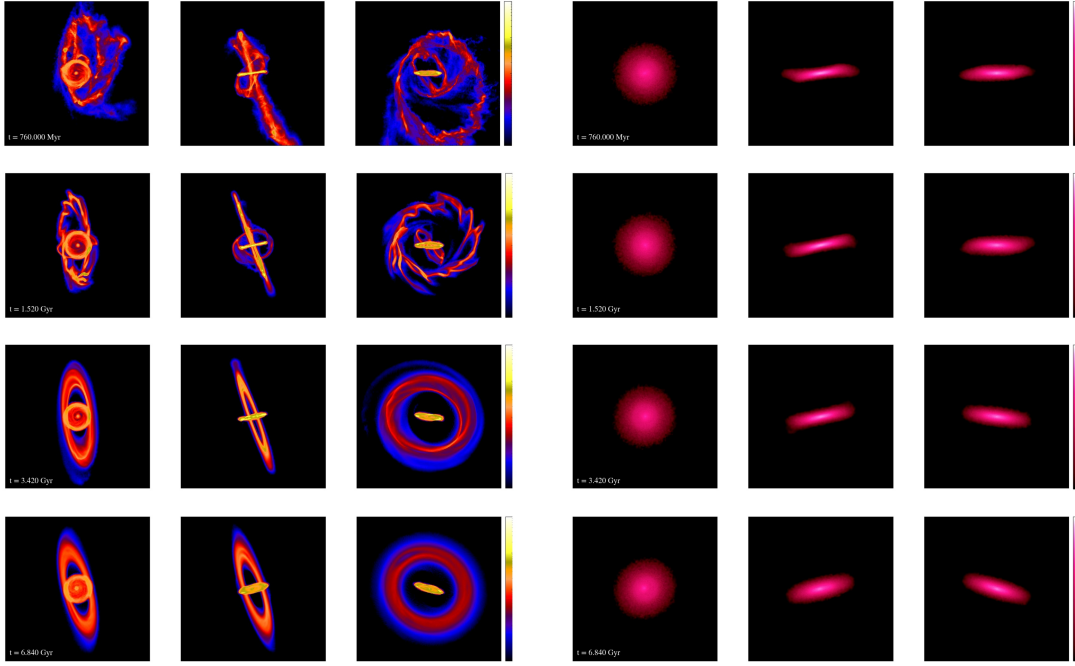
Fig. 2. Evolution of the polar gas ring in the galaxy over the time interval from 760 Myr to 6.84 Gyr. The gas subsystem of the galaxy (left) and the stellar disk (right) are shown. The frame has a size of 50 \times 50 kpc along each of the projections ( XY , XZ , YZ ). The range of variation of the surface density along the line of sight is within 1\text{--}10^4 M_{\odot}/\text{pc}^2 for the gas and \text{--}10\text{--}10^4 M_{\odot}/\text{pc}^2 for the stars.
