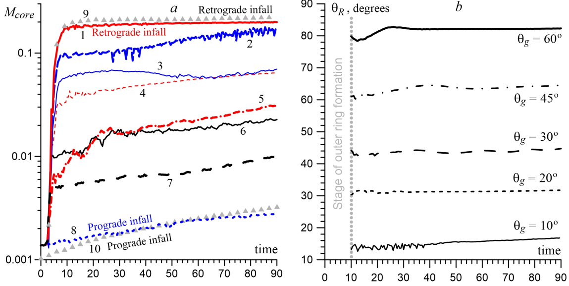
Fig. 3. a — Dependence of the gas mass inside 1 kpc for different angles of attack of the accreting intergalactic gas flow. Models of the bulgeless galaxy with retrograde infall (Khrapov & Khoperskov 2024): \Theta_g = 20^\circ (curve 1), \Theta_g = 10^\circ (2), \Theta_g = 5^\circ (3), \Theta_g = 30^\circ (4), \Theta_g = 40^\circ (5), \Theta_g = 45^\circ (6), \Theta_g = 60^\circ (7); prograde infall model at \Theta_g = 20^\circ (8); models with the bulge at \Theta_g = 20^\circ (curves 9 and 10). b — Outer gas ring tilt angles \Theta_R vs. time ( t ) for different \Theta_g .
