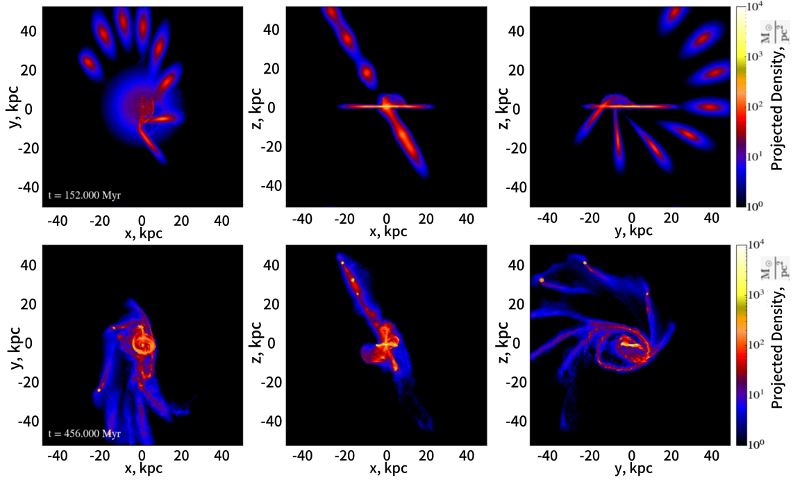
Fig. 1. Accretion of intergalactic gas onto a spiral galaxy in our numerical model. The moment of collision is shown in the top panel and the initial stage of polar ring formation is shown in the bottom panel (at \sim 300 Myr after the collision). Each frame has a size of 100 \times 100 kpc along each projection ( XY , XZ , YZ ). The range of variation of the surface gas density along the line of sight is 1\text{--}10^4 M_{\odot}/\text{pc}^2 .
